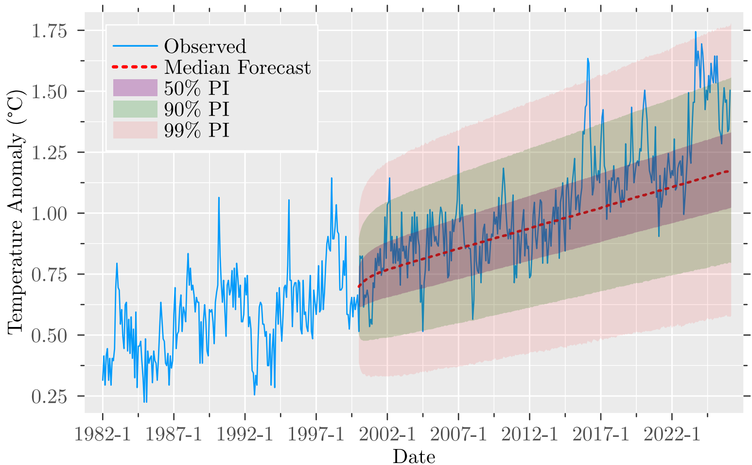
Forecasted Temperature with PI (GISTEMP)
