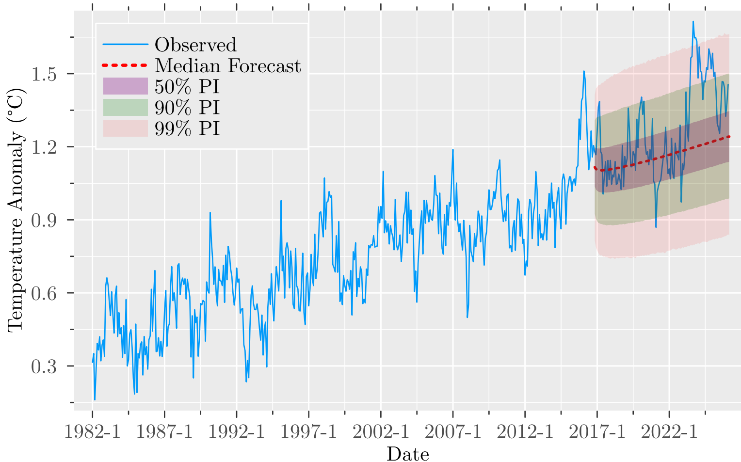
Forecasted Temperature with PI (Berkeley)
