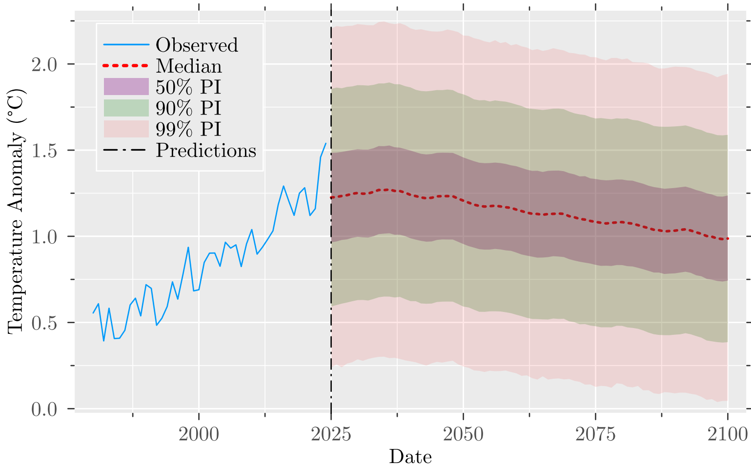
Forecasted Temperature with PI (SSP1-1.9)
