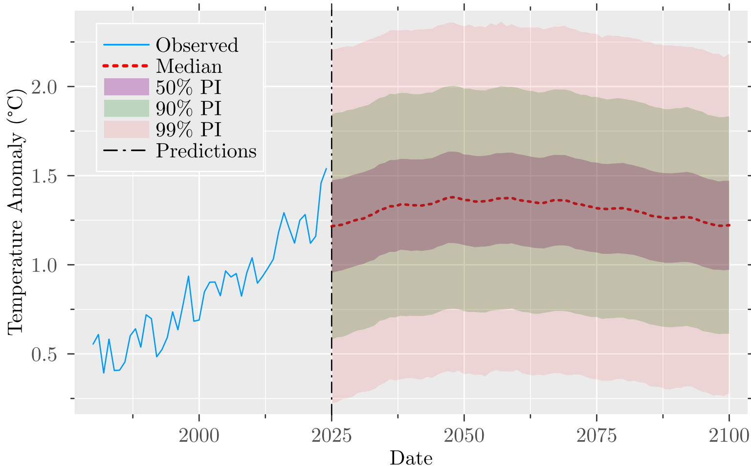
Forecasted Temperature with PI (SSP1-2.6)
