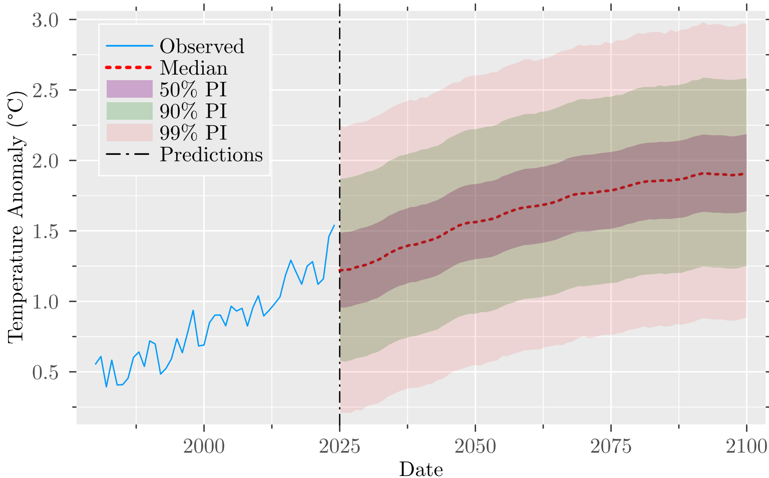
Forecasted Temperature with PI (SSP2-4.5)
