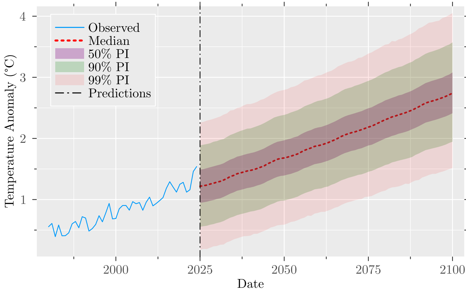
Forecasted Temperature with PI (SSP3-7.0)
