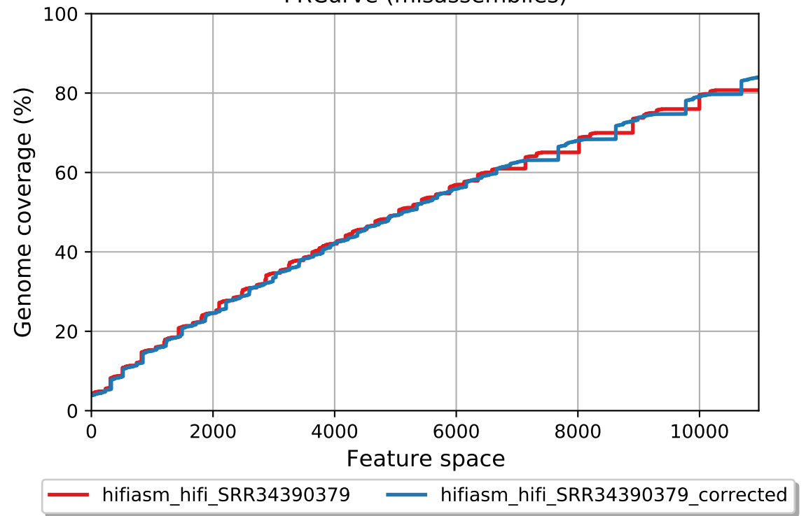
FRCurve (misassemblies)
