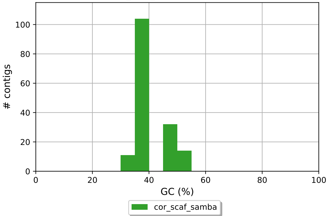
cor_scaf_samba GC content
