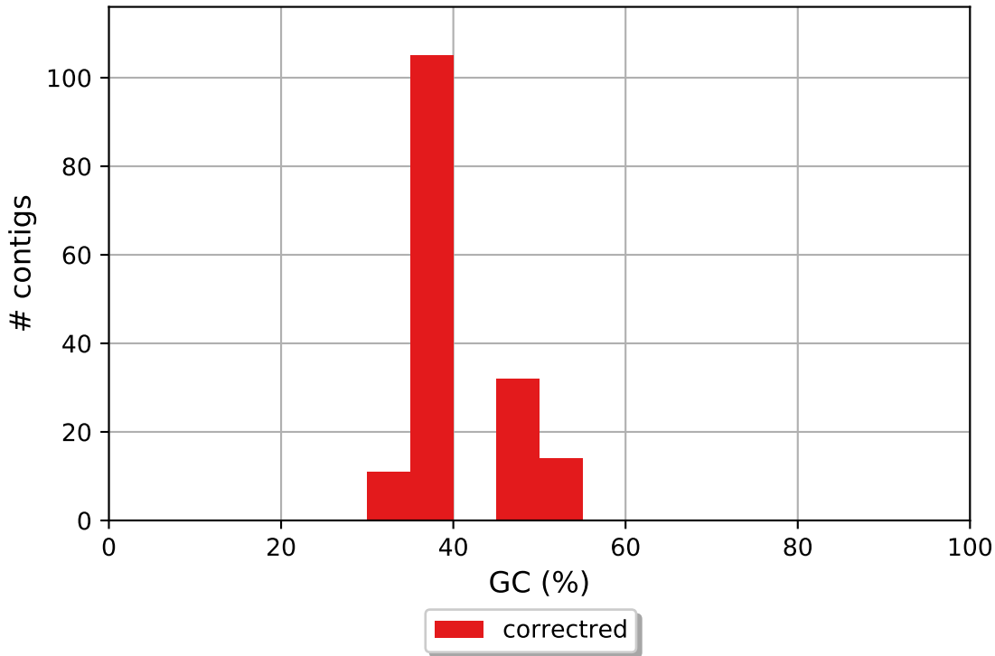
correctred GC content
