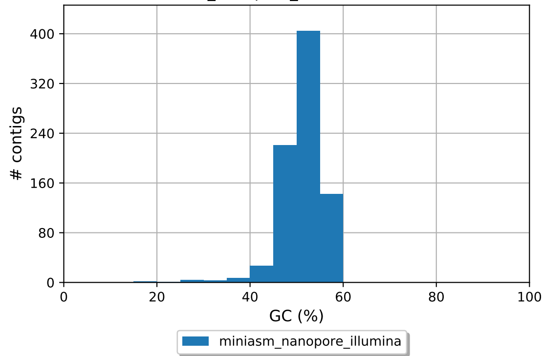
miniasm_nanopore_illumina GC content
