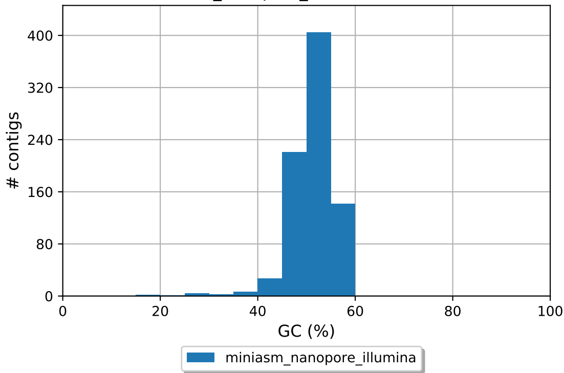
miniasm_nanopore_illumina GC content
