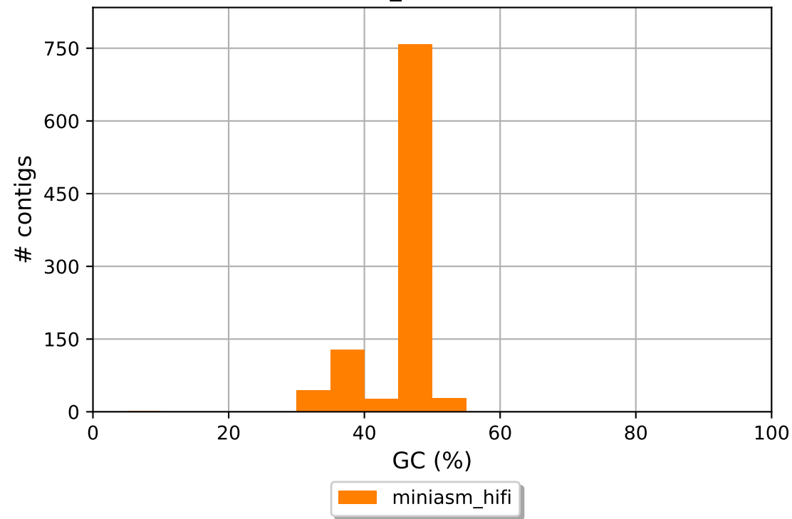
miniasm_hifi GC content
