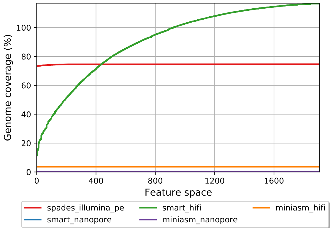
FRCurve (misassemblies)
