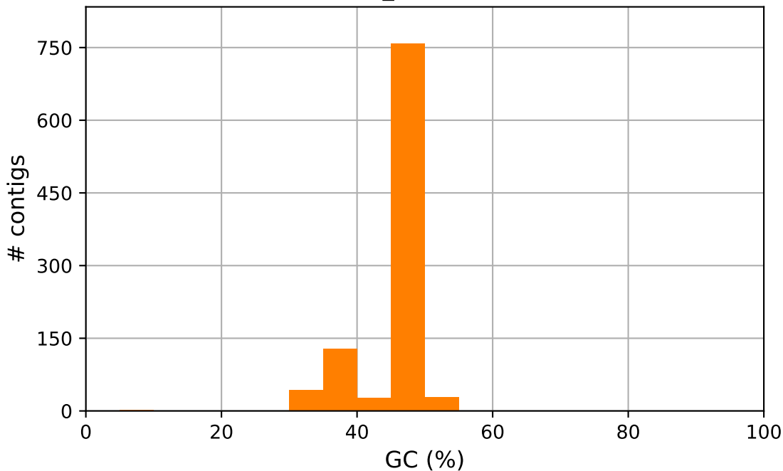
miniasm_hifi GC content
