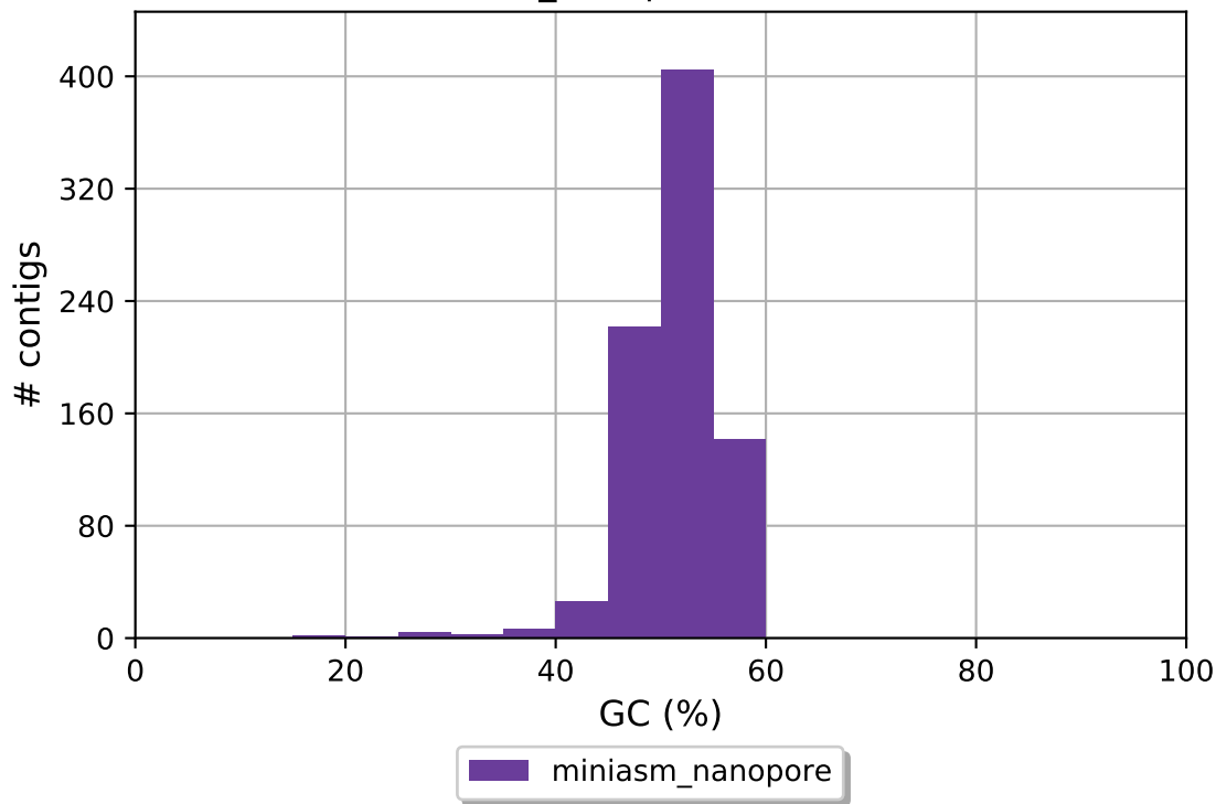
miniasm_nanopore GC content
