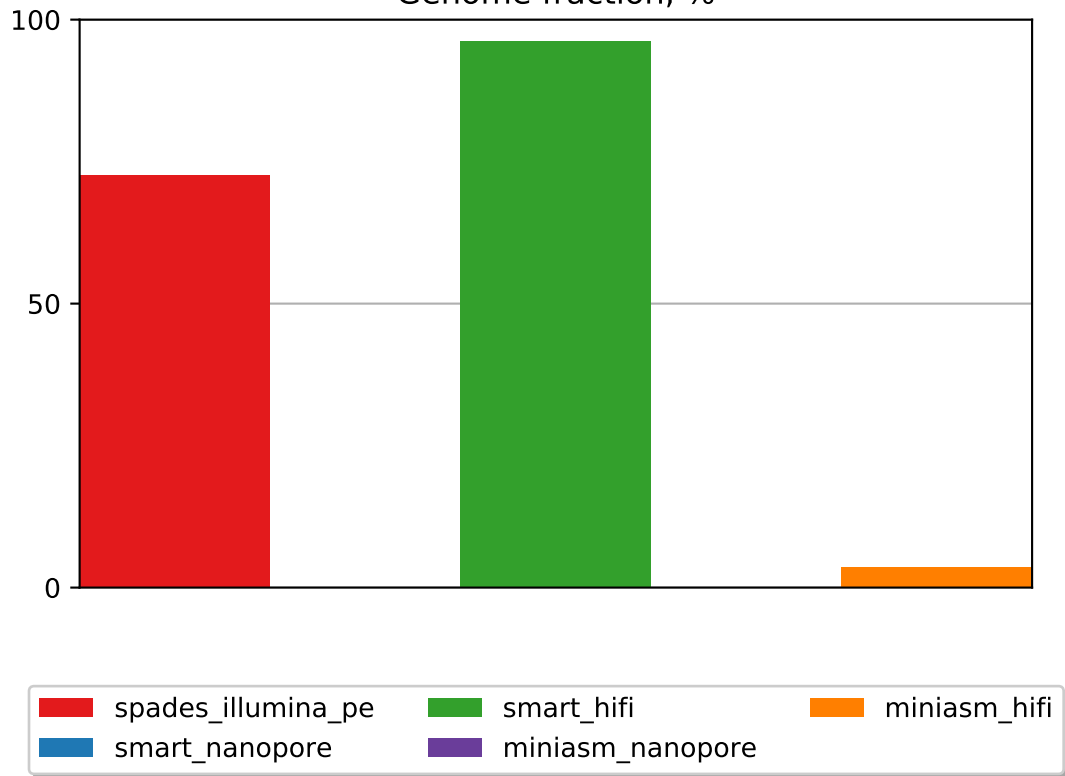
Genome fraction, %
