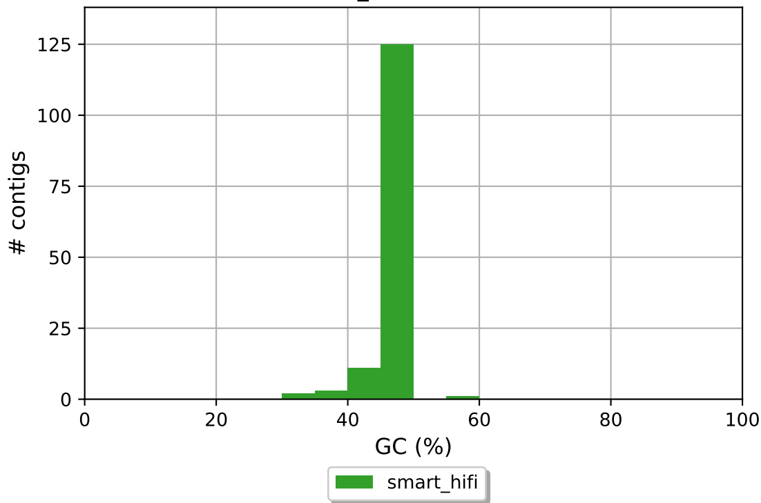
smart_hifi GC content
