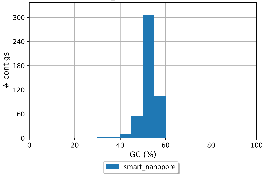
smart_nanopore GC content
