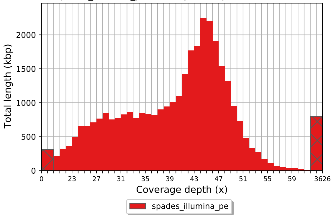
spades_illumina_pe coverage histogram (bin size: 1x)
