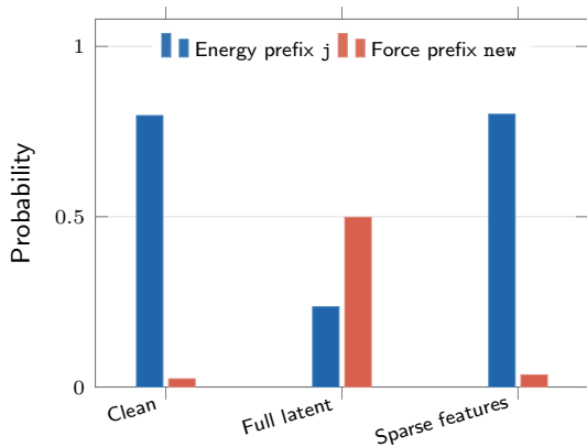
(a) Energy target: answer-prefix probabilities
