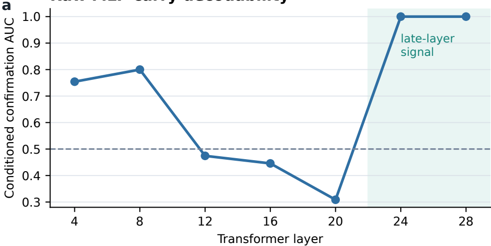
a Raw MLP carry decodability
