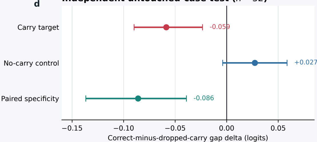
d Independent untouched-case test ( n = 32 )
