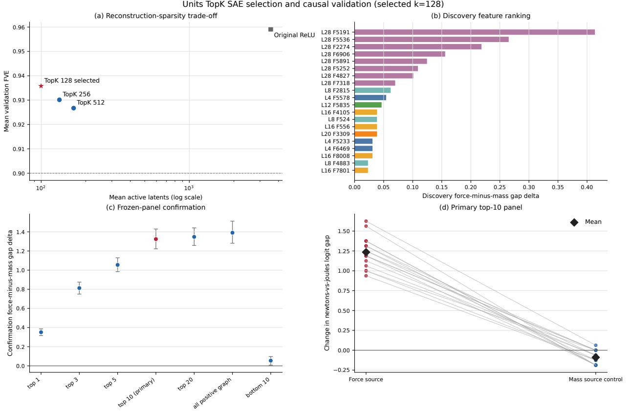
Figure 8: Units TopK selection, discovery ranking and frozen confirmation. Panel (a) shows the reconstruction-sparsity criterion that selected TopK-128 before intervention. Panel (b) ranks graph features by the discovery force-minus-mass effect, with the first ten forming the frozen panel. Panel (c) compares cumulative panel sizes with the full positive graph and reverse-ranked control. Panel (d) shows paired confirmation effects for all 16 systems; every force-source shift exceeds its mass-source control.
