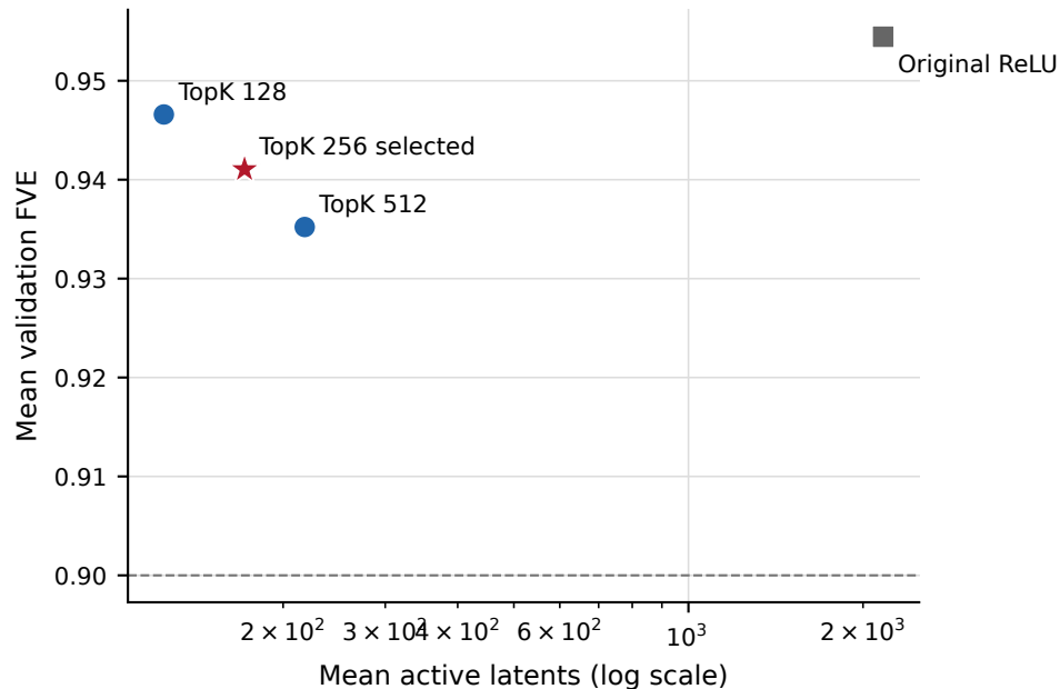
(a) Reconstruction-sparsity trade-off
