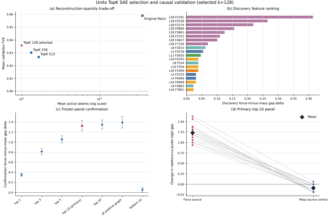
Figure 9: Units TopK selection, discovery ranking and frozen confirmation. Panel (a) shows the reconstruction-sparsity criterion that selected TopK-128 before intervention. Panel (b) ranks graph features by the discovery force-minus-mass effect, with the first ten forming the frozen panel. Panel (c) compares cumulative panel sizes with the full positive graph and reverse-ranked control. Panel (d) shows paired confirmation effects for all 16 systems; every force-source shift exceeds its mass-source control.
