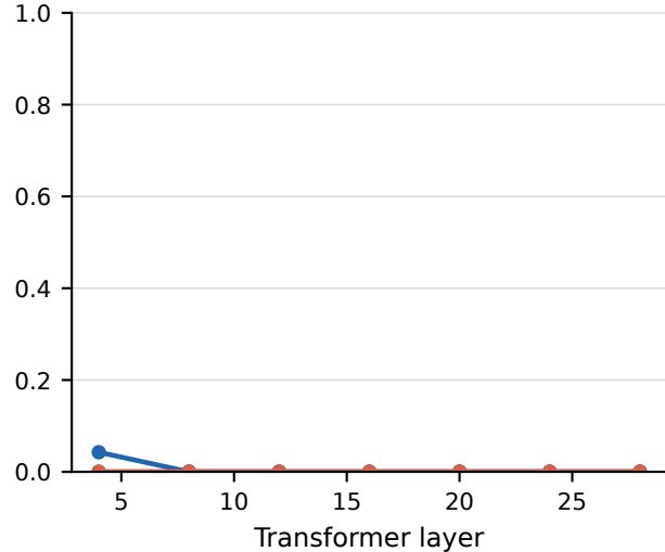
Dead-feature fraction
