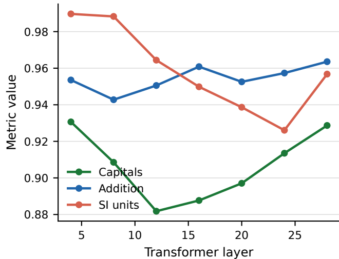
Validation FVE
