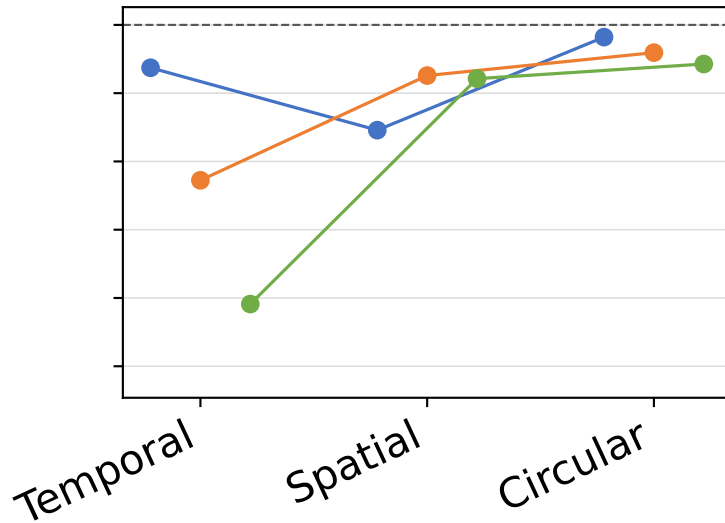
Miller-Madow
