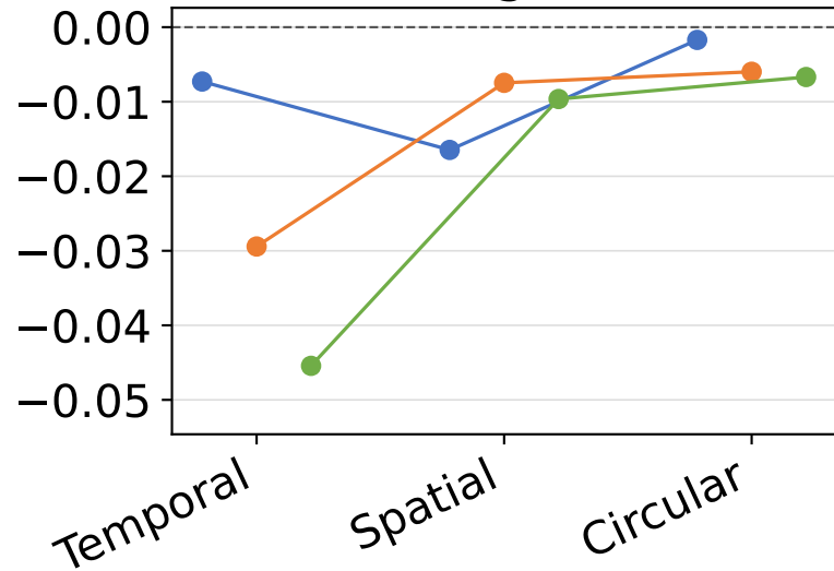
Plug-in
