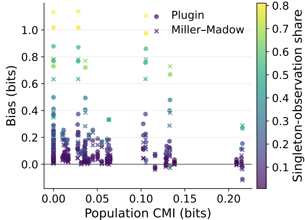
(a) Bias across null and alternatives
