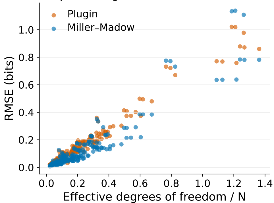
(b) Sparse degrees of freedom and RMSE
