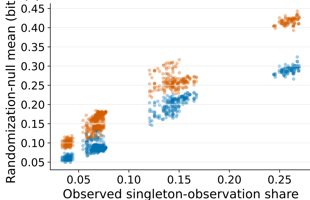
(c) A randomization null need not center at zero
