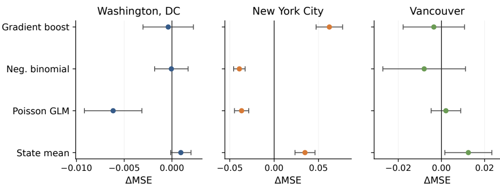
Figure 9. Held-out integer-MSE change after adding lagged bicycle state. Positive values favor the bicycle-augmented specification; comparisons are paired within city and model family.
