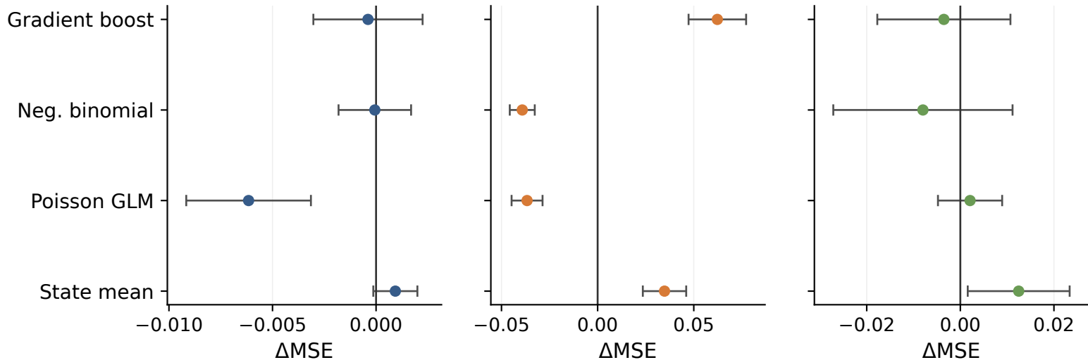
Washington, DC
