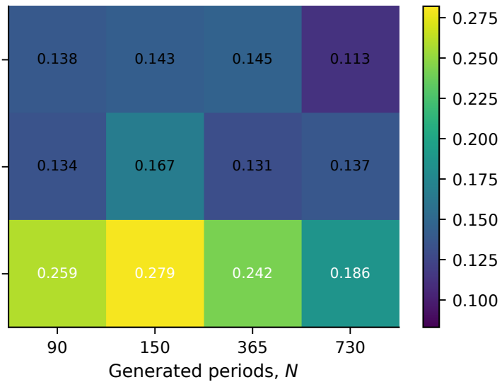
(c) Jeffreys-Dirichlet
