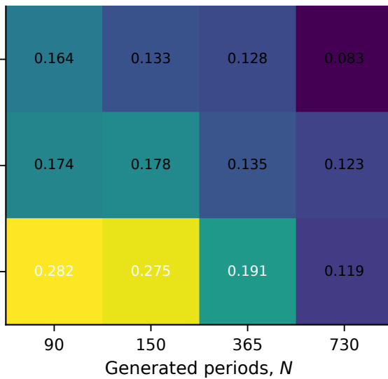
(b) Miller-Madow
