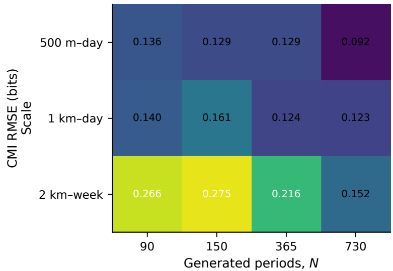
(a) Plugin
