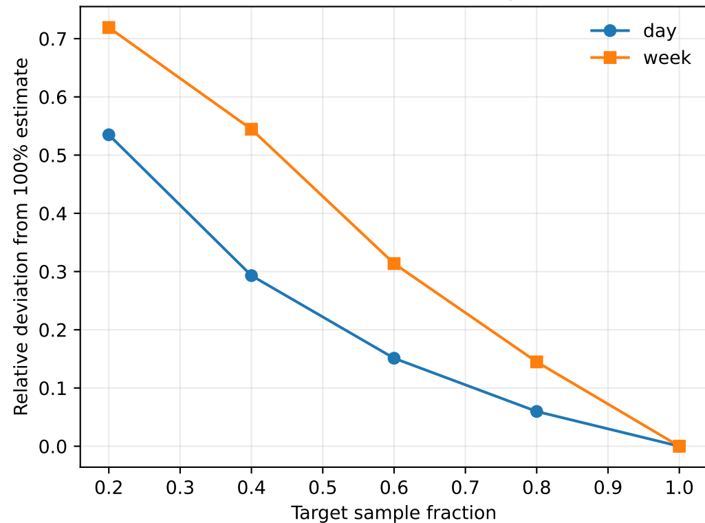
Baseline DELB stability
