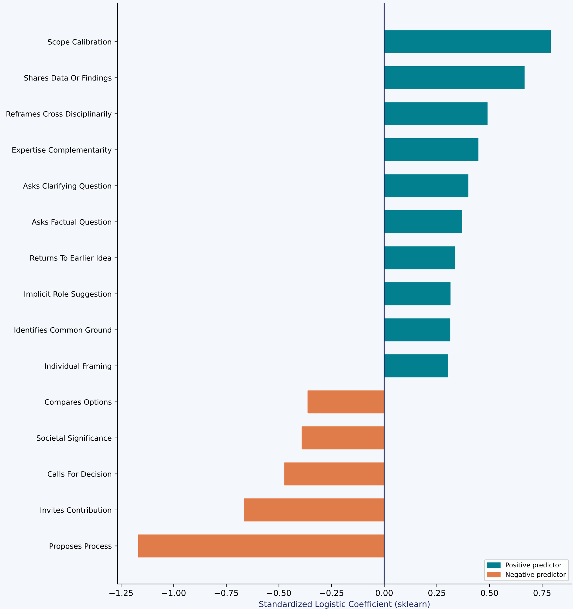
Top Behaviors in Last 5 min LOCO-CV: AUC=0.810 AUPRC=0.803 (n=579, non-fac) (top 15 subcodes by |coef|, trained on full non-fac sample)
