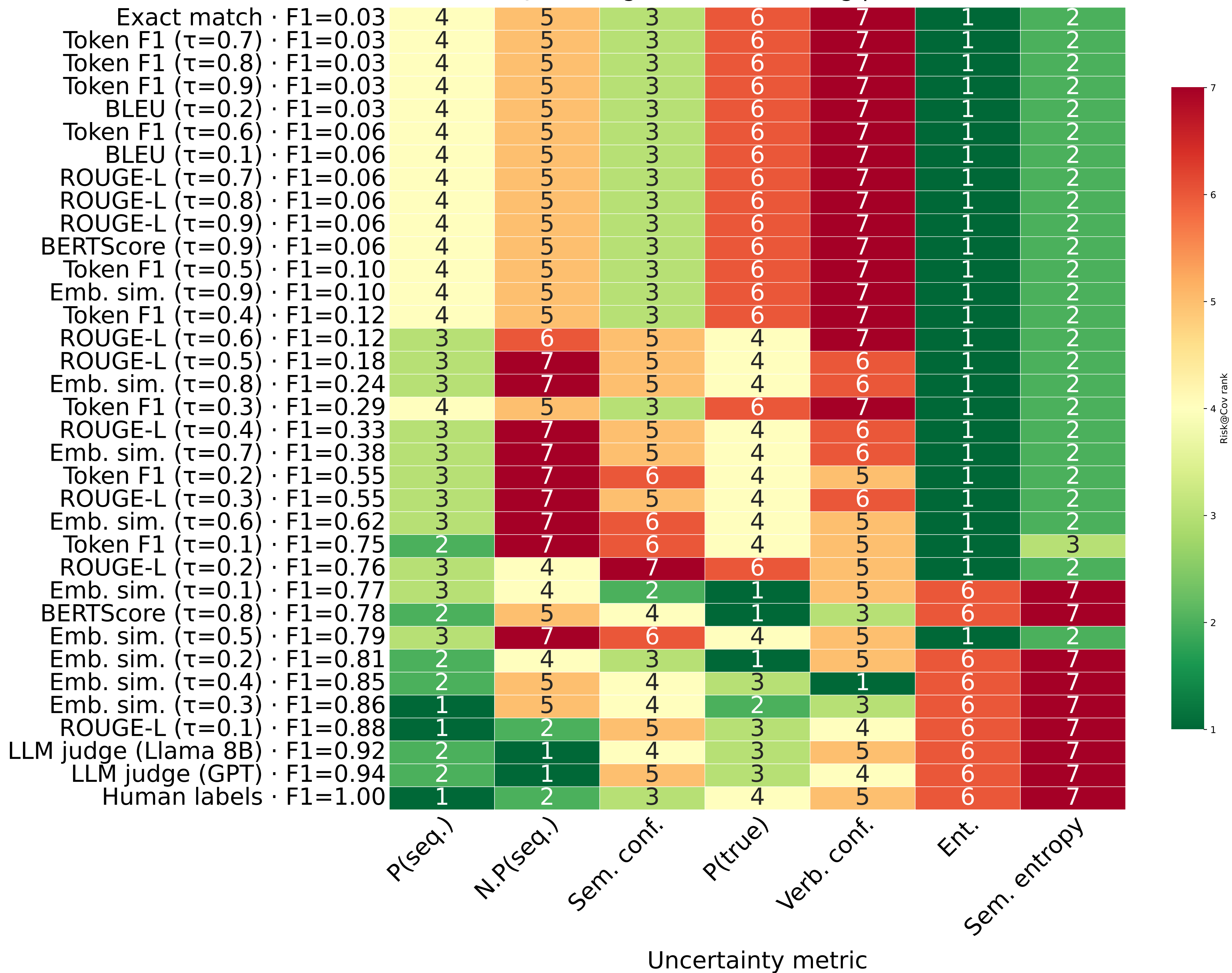
Risk@Coverage (80.0%) Ranking per Correctness
