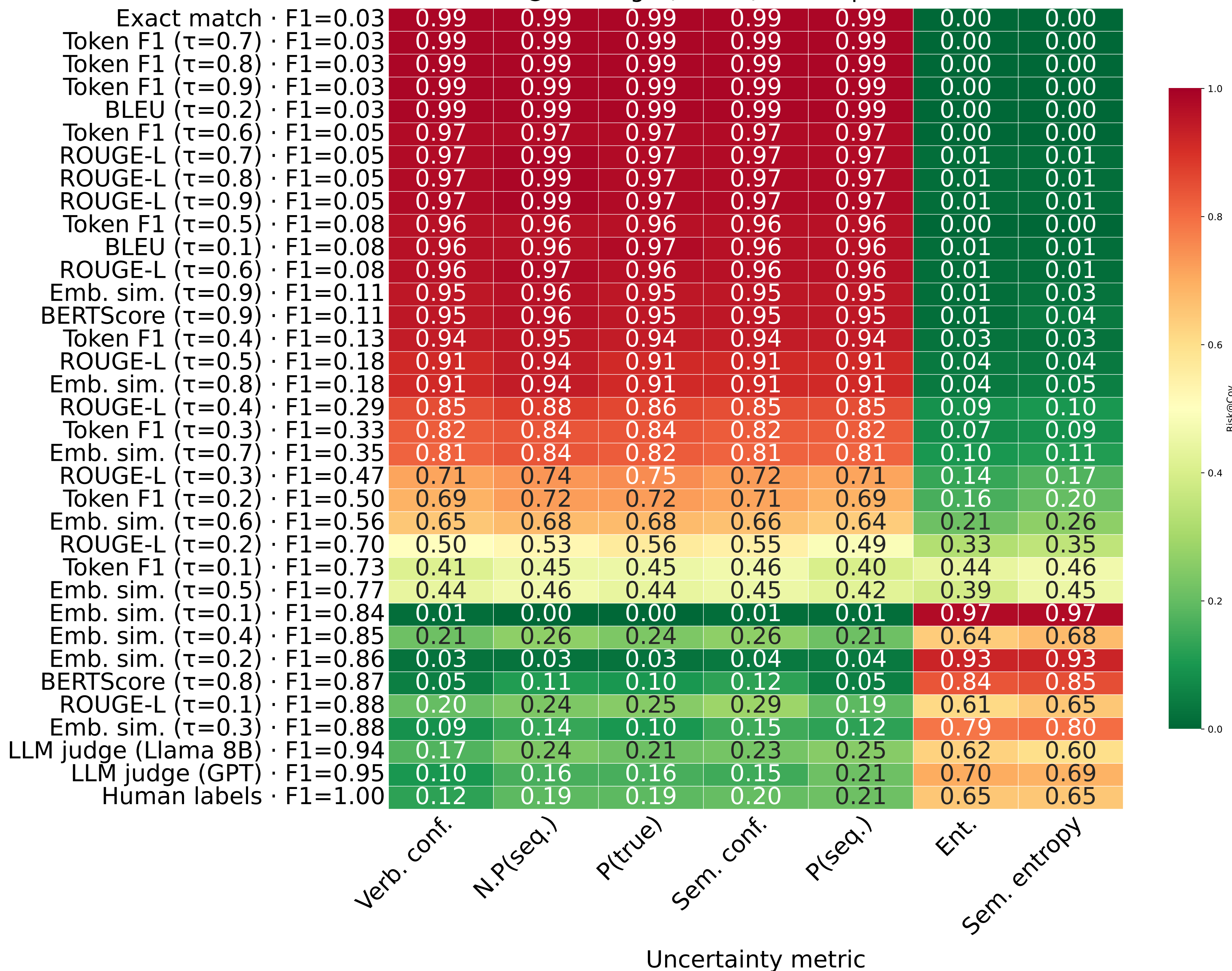
Risk@Coverage (80.0%) Values per Correctness
