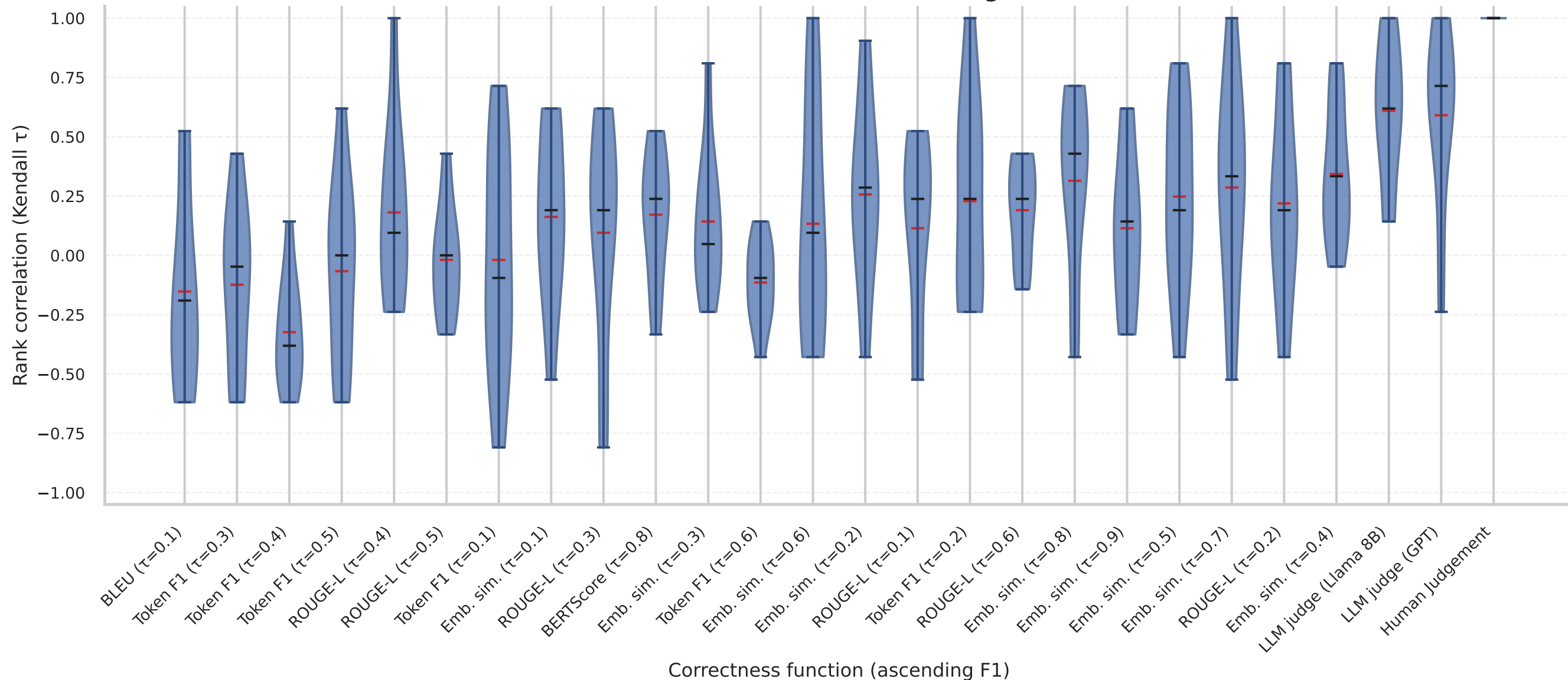
Manual vs automated AUROC ranking correlation
