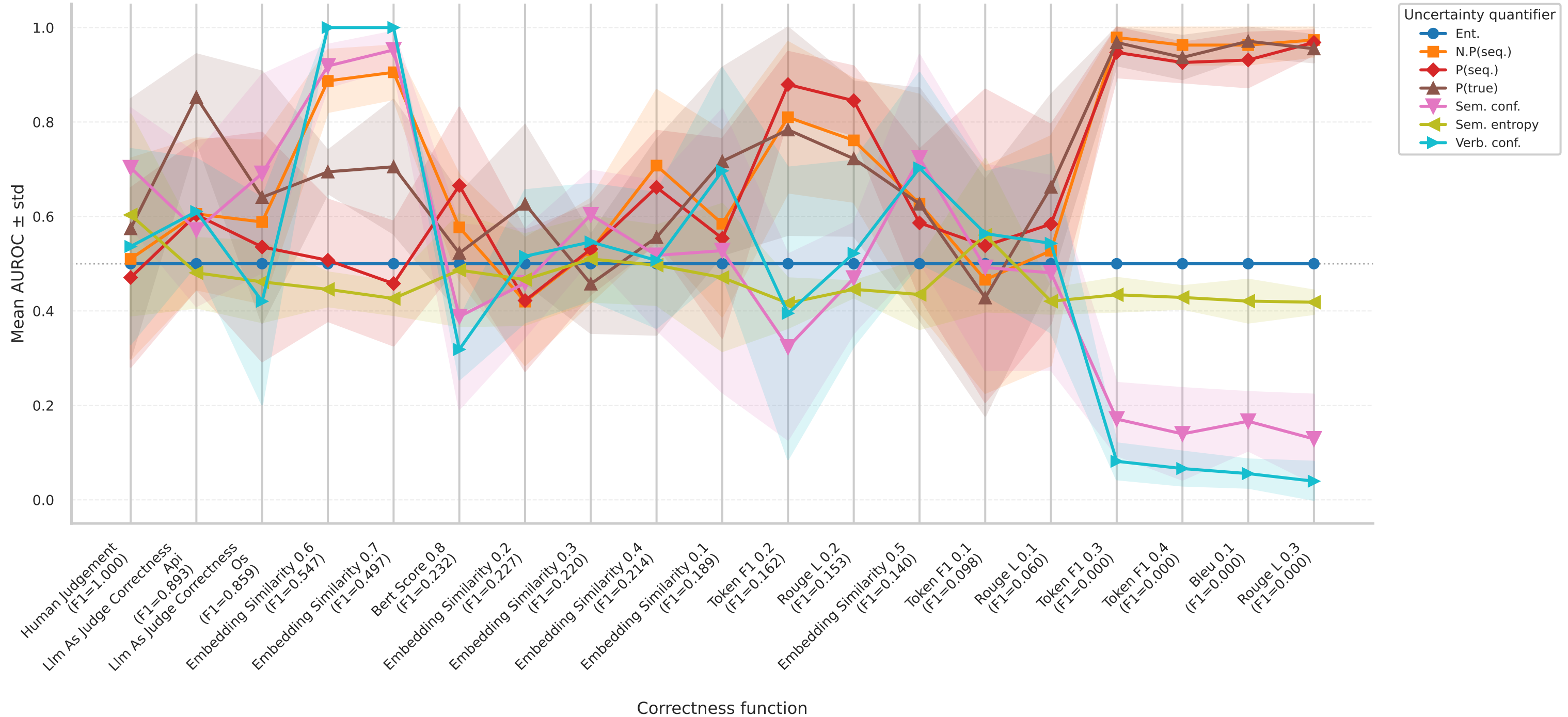
Mean AUROC across correctness functions
