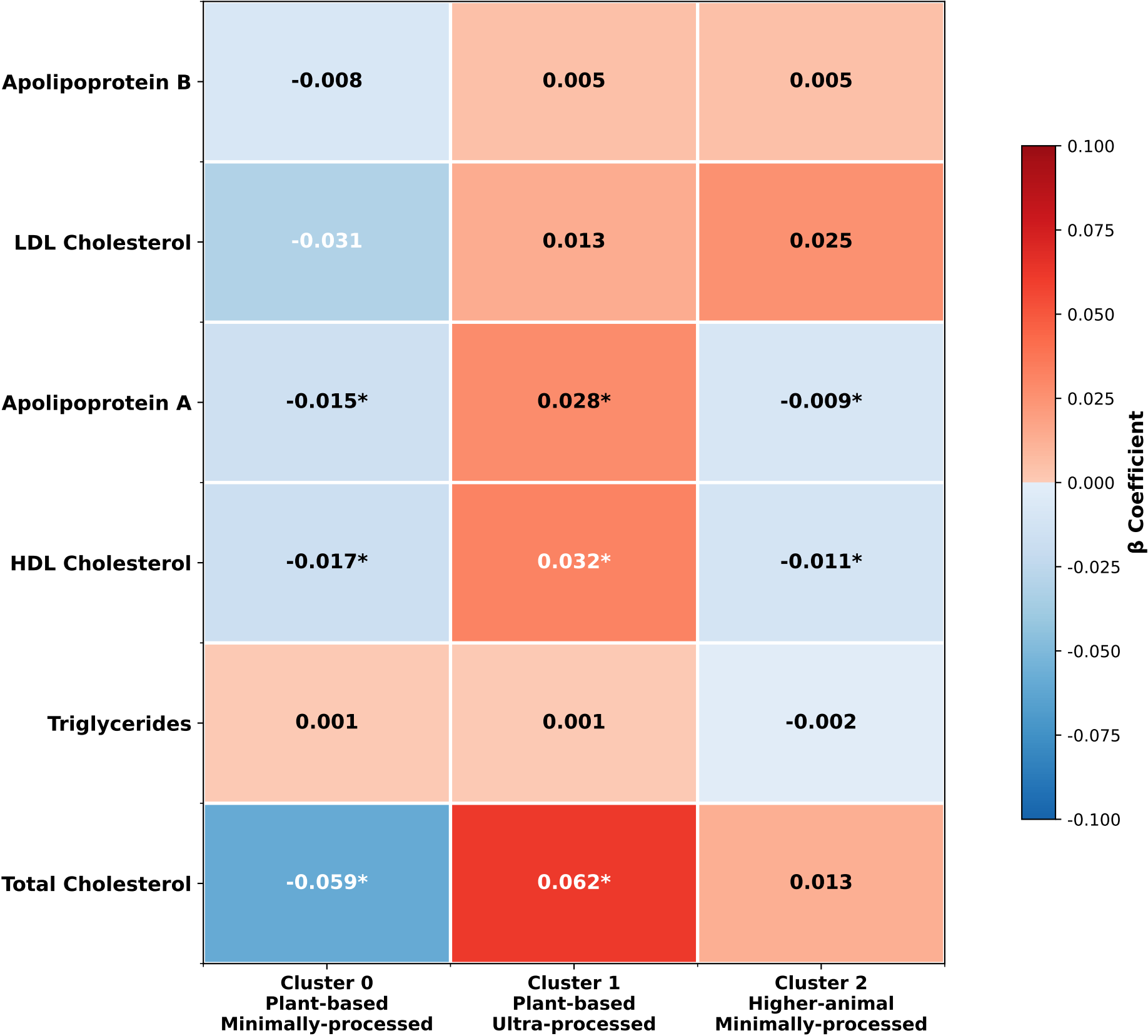
β Coefficient Heatmap (Lipid ~ Diet Cluster Associations, * = FDR < 0.05)
