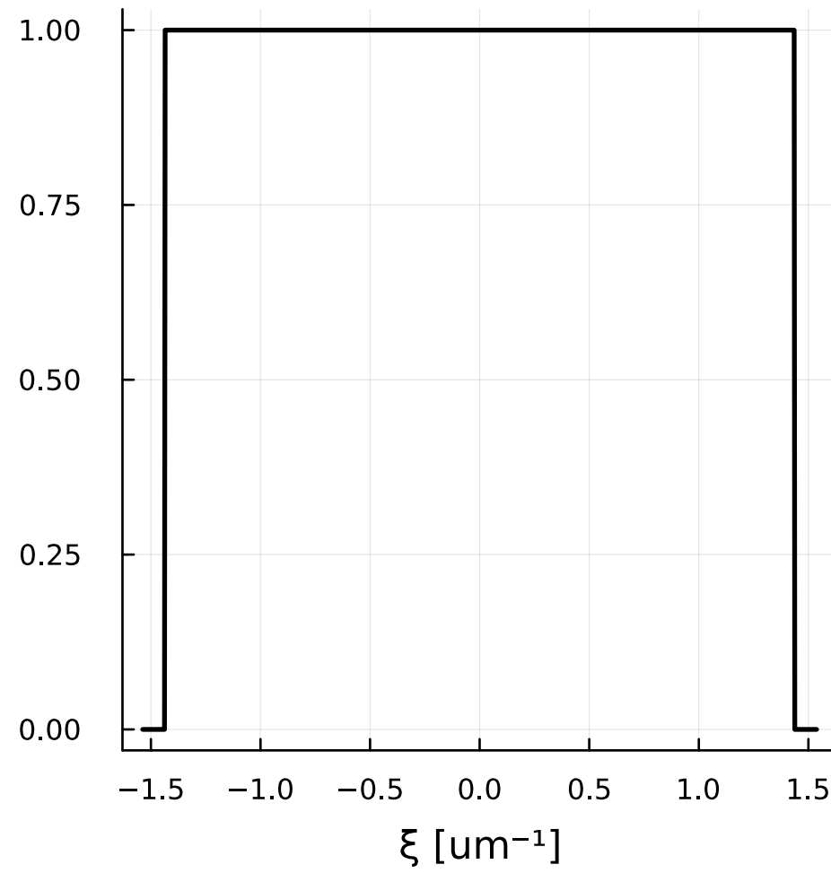
Nyquist filter (x=0)
