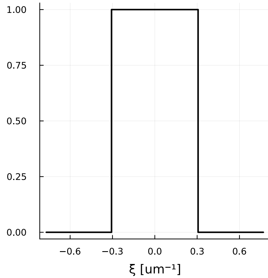
Nyquist filter (x=0)
