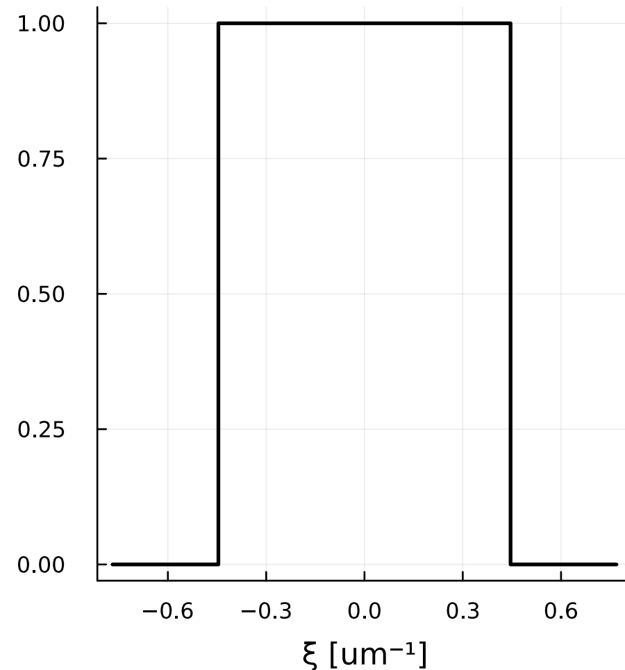
Nyquist filter ( x=0 )
