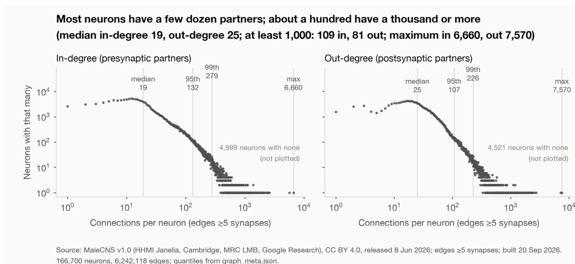
Figure 2: In-degree and out-degree of the built graph on log-log axes, two small multiples at one scale. Quantiles from data/malecns/graph_meta.json are marked on the axes; 109 neurons have in-degree of 1,000 or more and 81 have out-degree of 1,000 or
