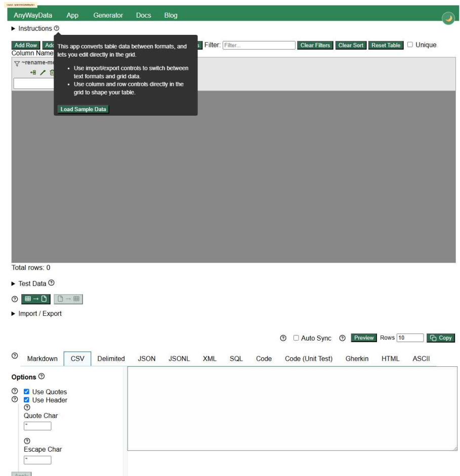
Figure 1: Browser proof
