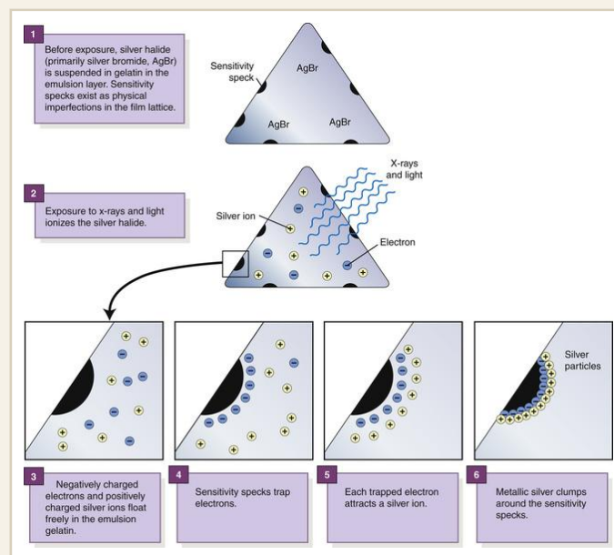
HOW LIGHT WRITES: THE GURNEY-MOTT MECHANISM OF LATENT-IMAGE FORMATION. (FAUBER, RADIOGRAPHIC IMAGING & EXPOSURE)
