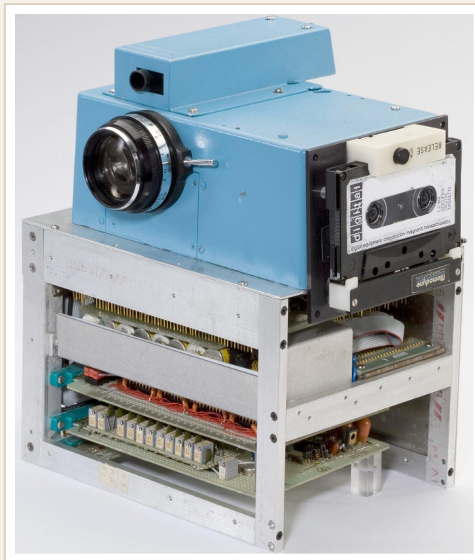
STEVEN SASSON'S 1975 PROTOTYPE: LENS, CCD, AND A CASSETTE DECK. PHOTO: EASTMAN KODAK, VIA THE NEW YORK TIMES.
