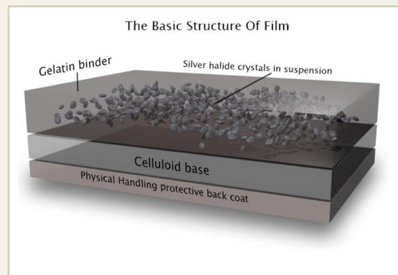
THE STRUCTURE OF FILM: A GELATIN EMULSION HOLDING SILVER-HALIDE CRYSTALS, COATED ON THE BASE.
