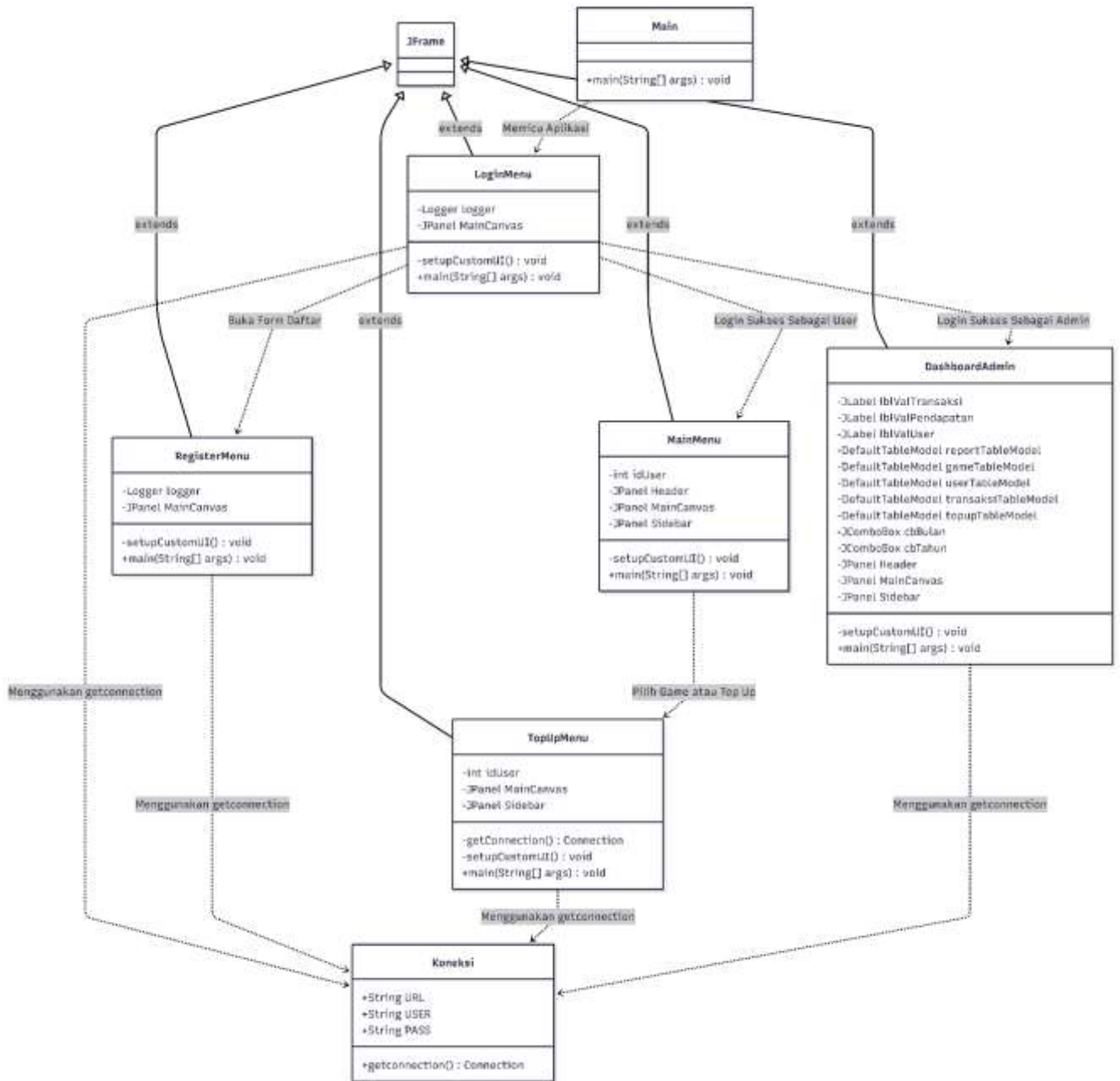
Gambar 2. 6 Class Diagram
