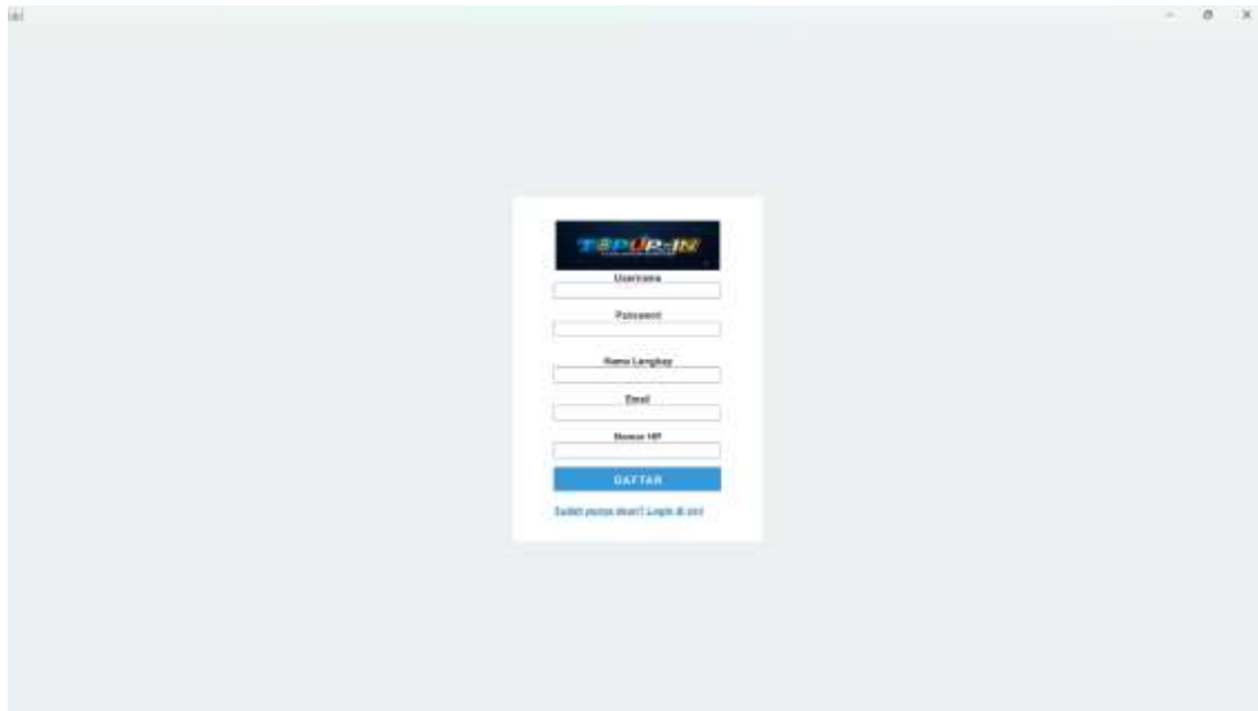
Gambar 2. 9 UI Register
