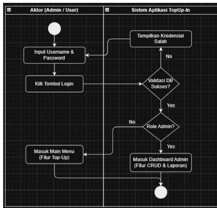
Gambar 2. 2 Activity Diagram
