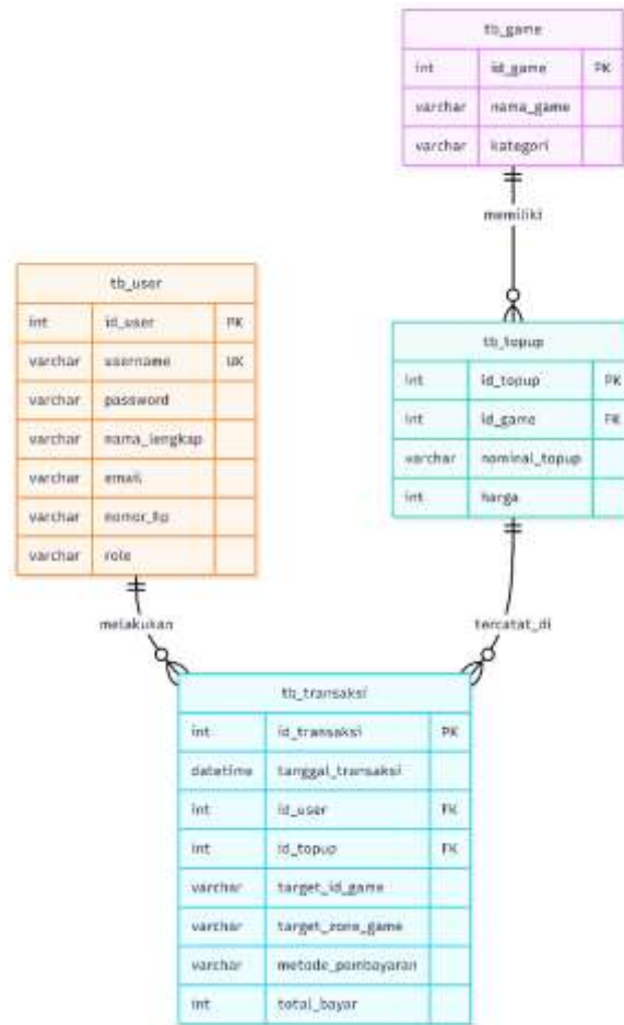
Gambar 2. 7 Entity Relationship Diagram
