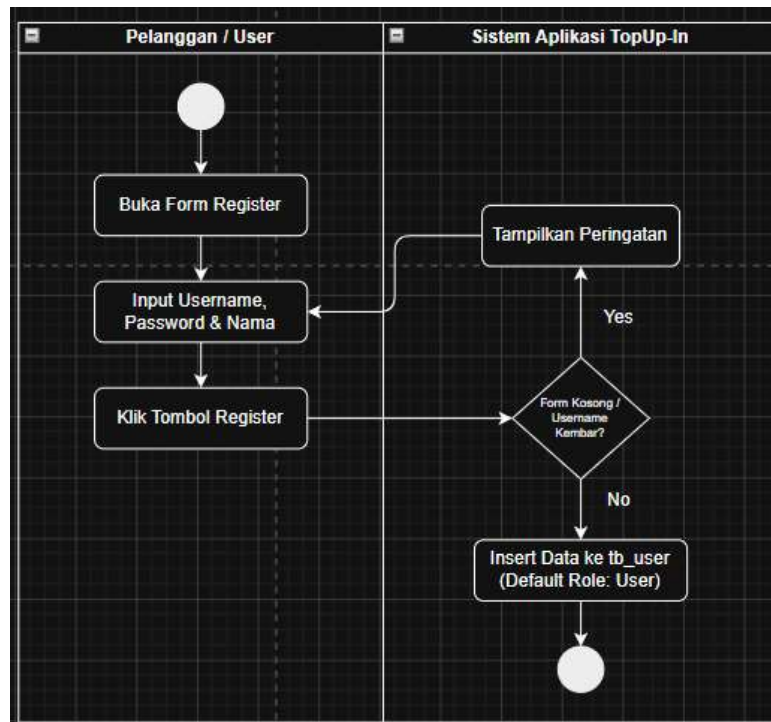
Gambar 2. 3 Register
