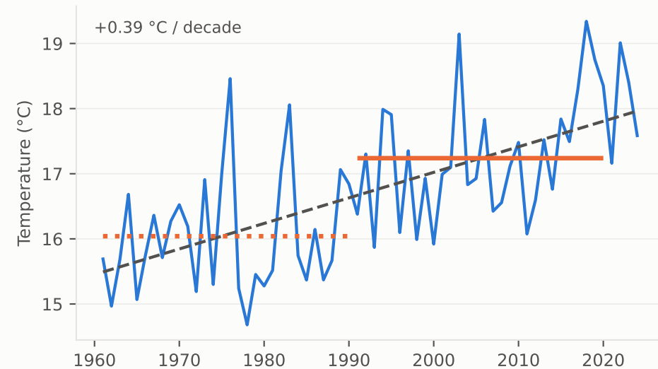
Summer (JJA) +1.20 °C between normals
