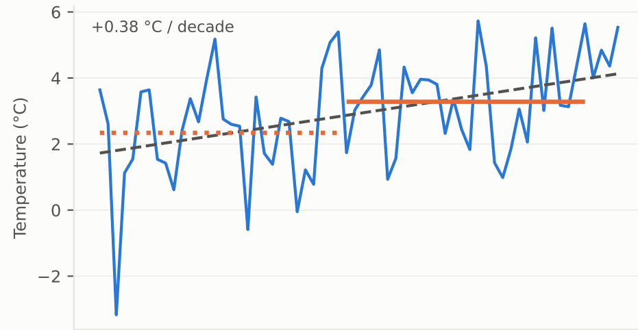
Winter (DJF) +0.94 °C between normals
