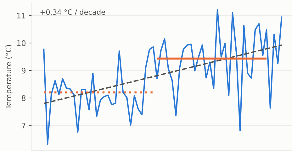
Spring (MAM) +1.23 °C between normals
