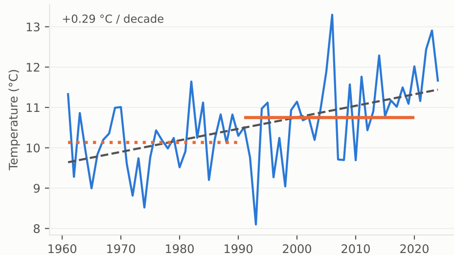
Autumn (SON) +0.62 °C between normals
