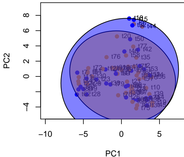
PCoA: Euclidean (m2)
