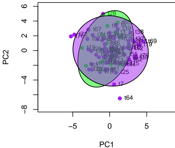
PCoA: Euclidean (m3)
