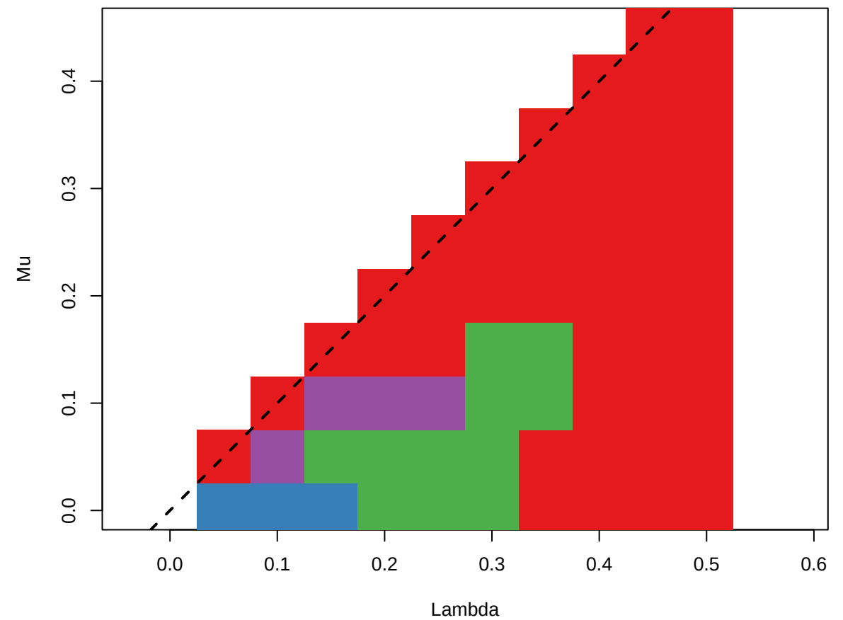
Shape Classes (rho = 0.6 )
