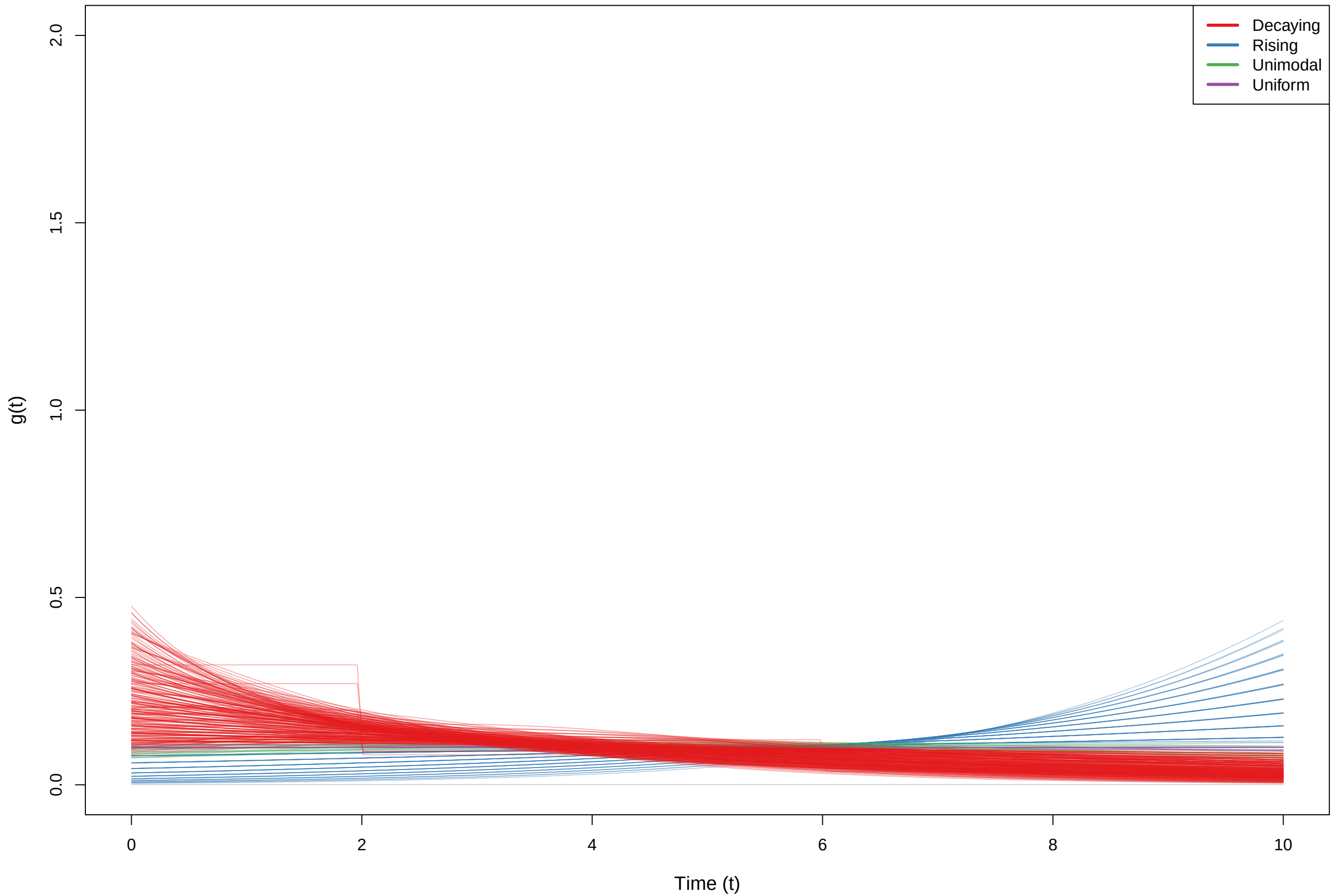
BD Density Functions Colored by Shape Class (root_age = 10)
