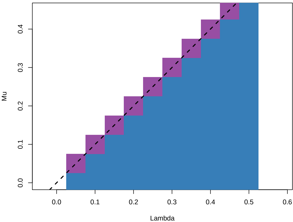
Shape Classes (rho = 0.4 )
