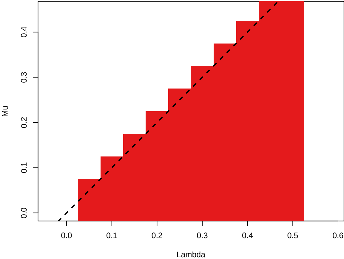
Shape Classes (rho = 0.8 )
