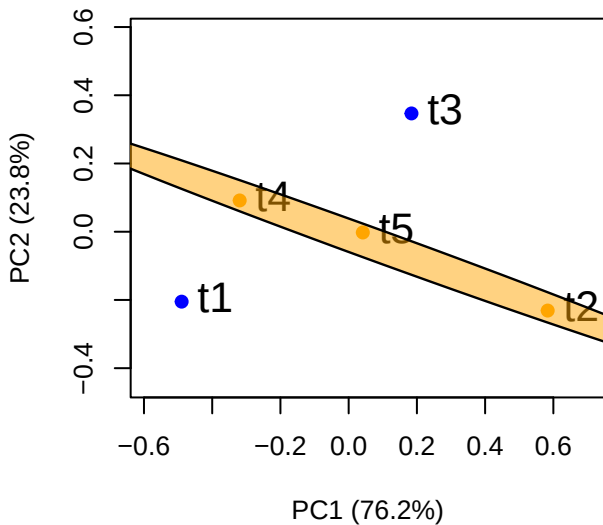
PCoA: Euclidean (CLR, phylo decorrelated)
