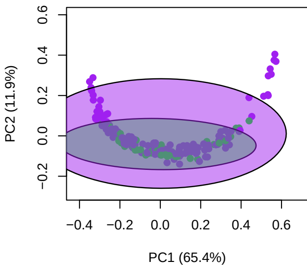
PCoA BC-distance
