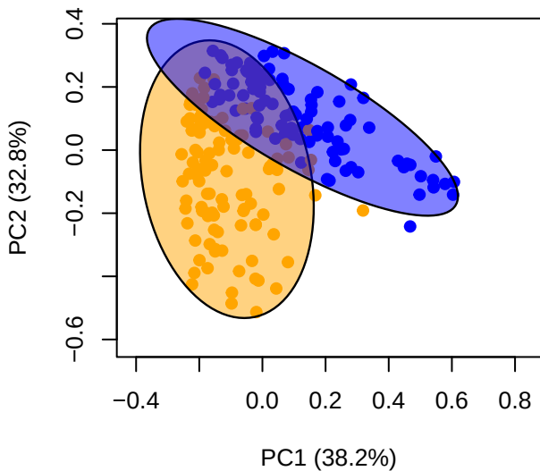
PCoA BC-distance
