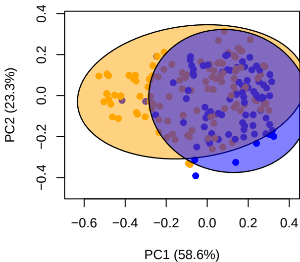
PCoA BC-distance
