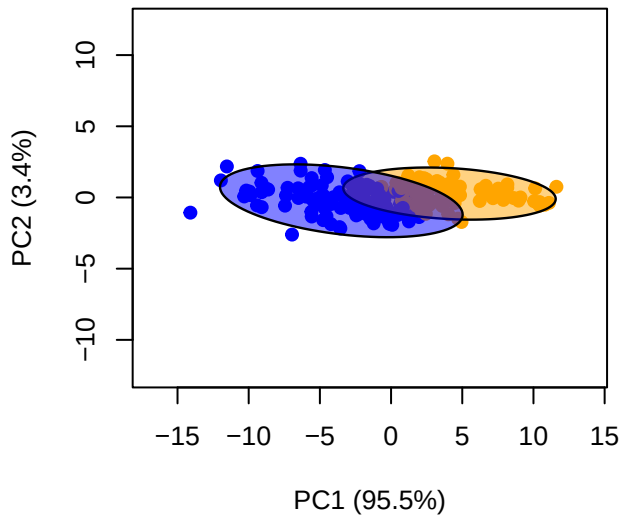
PCoA: Euclidean (CLR, standard)
