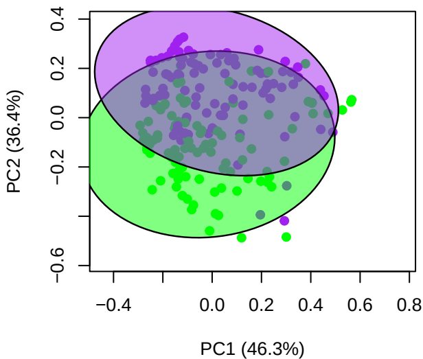
PCoA BC-distance
