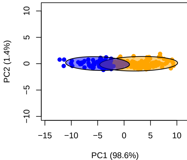
PCoA: Euclidean (CLR, standard)
